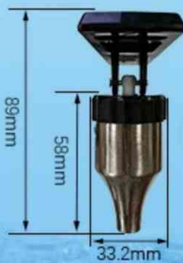
TY-147 Male
