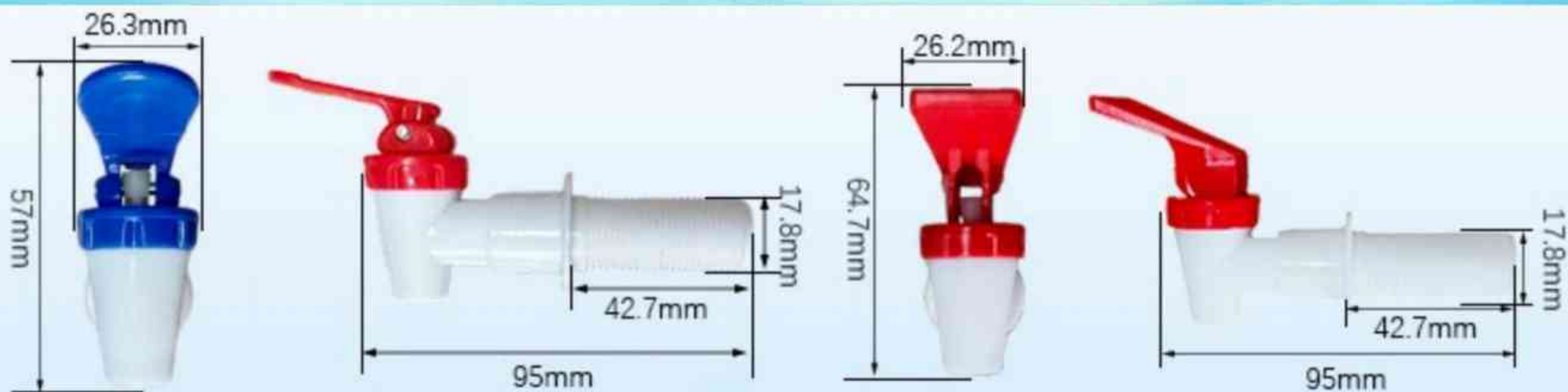
TY-075 Male
