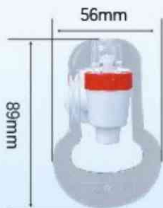
TY-003 Male
