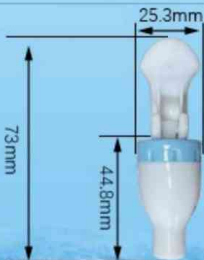
TY-102-2 Male
